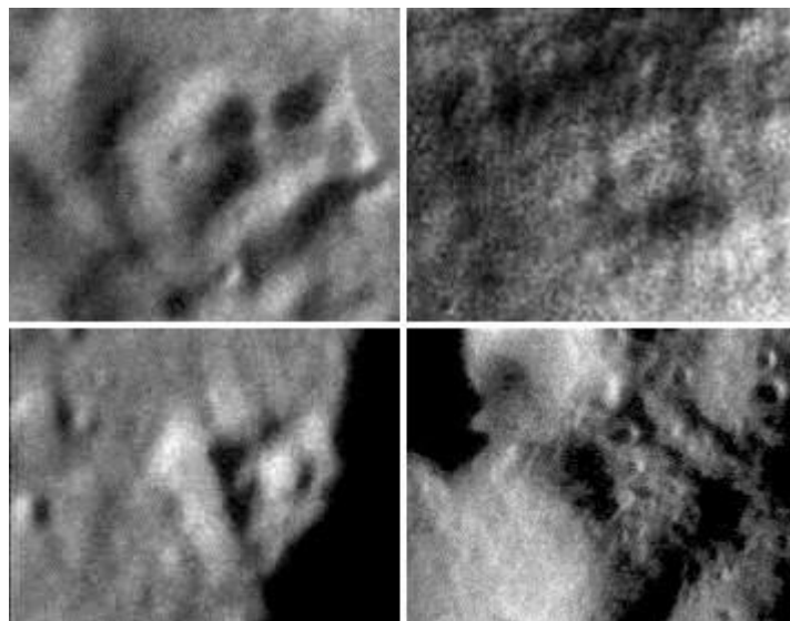
Fig. 6 The SAAM processing reveals the lattice pattern on the HIRES image LHD5165R.171.
