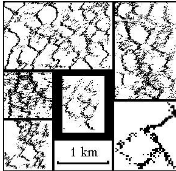
Fig. 10 Hidden rectangular patterns on the schemes (local extremities of relief) of HIRES images LHD0146A.210, LHD0331A.062, LHD0558B.072, LHD4691Q.253, LHD5243Q.208, and LHD6158R.320.
