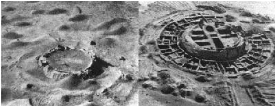
Fig. 1 The ancient Khorezmian fortress Koy-Krylgan-kala appeared as an impact crater on the air photo (left); its artificiality is obvious after the excavations in 1956 (right) [6].
